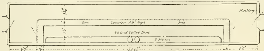
PLAN OF PERE MARQUETTE LUNCH COUNTER CAR.
